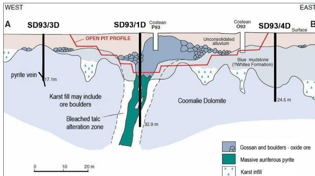
Figure 2 Sundance Prospect cross-section with lithology
